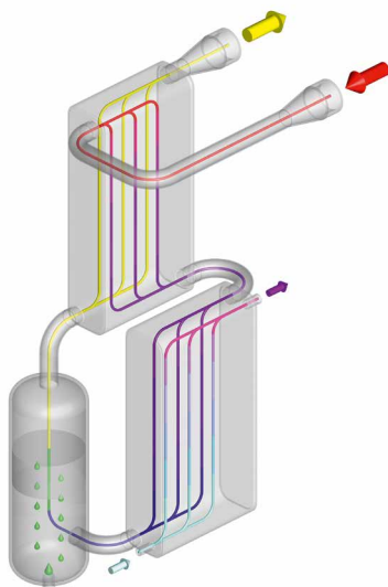
Stainless steel plate heat exchanger
