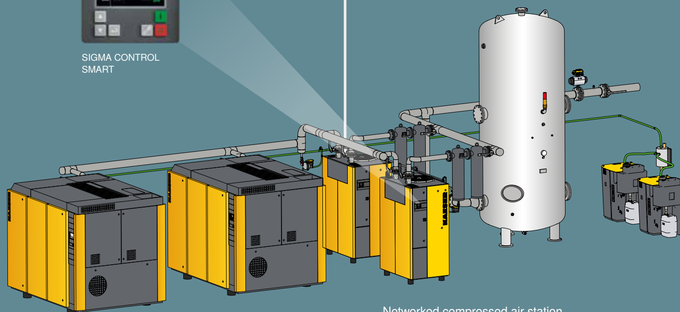
Networked compressed air station
