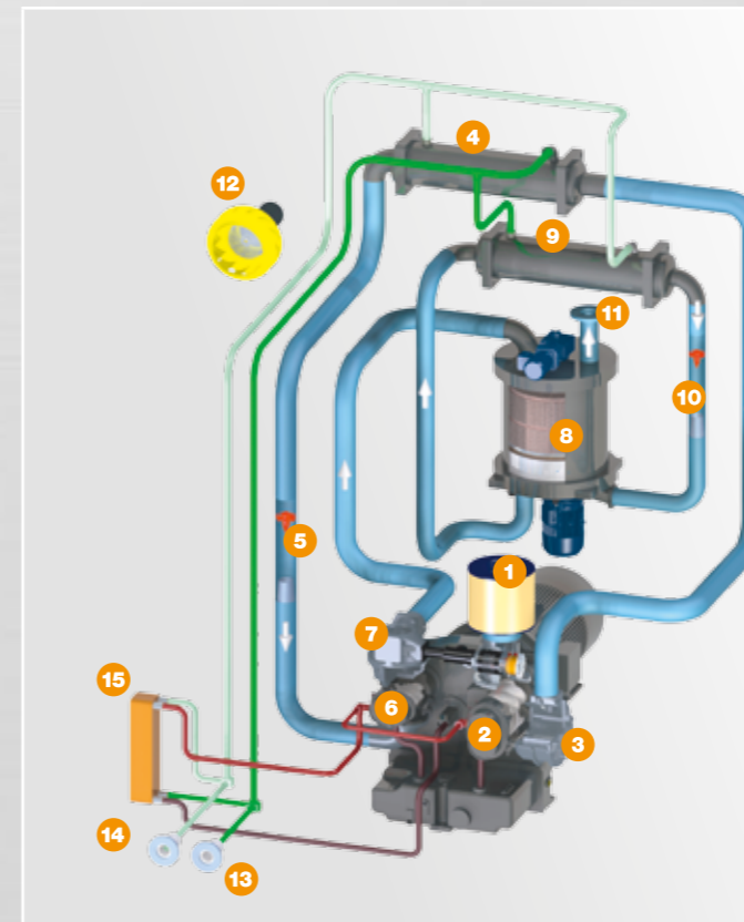
Image: Standard version DSG-2 RD, water-cooled
